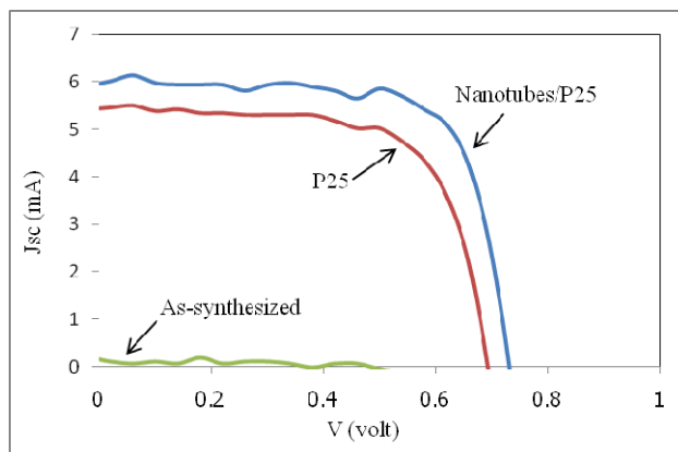
Fig. 7 Photocurrent–voltage characteristic of a typical dye sensitized solar cells fabricated by the as-synthesized sample, the mixed of nanotubes-nanoparticles and P-25 and P-25.
