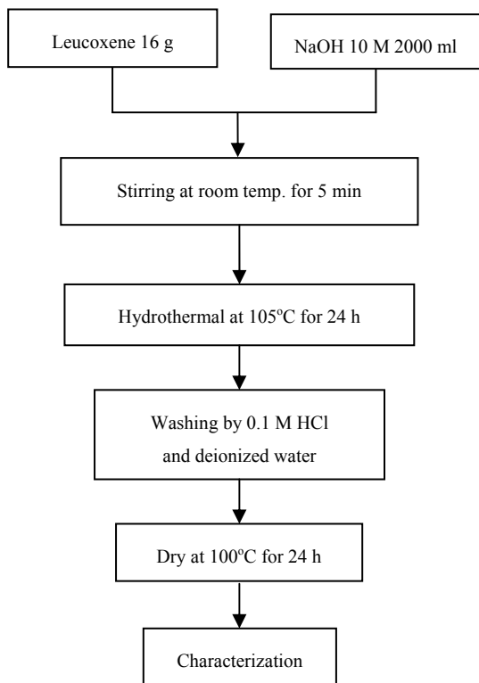
Fig. 2. Schematic representation for experimental procedure.
