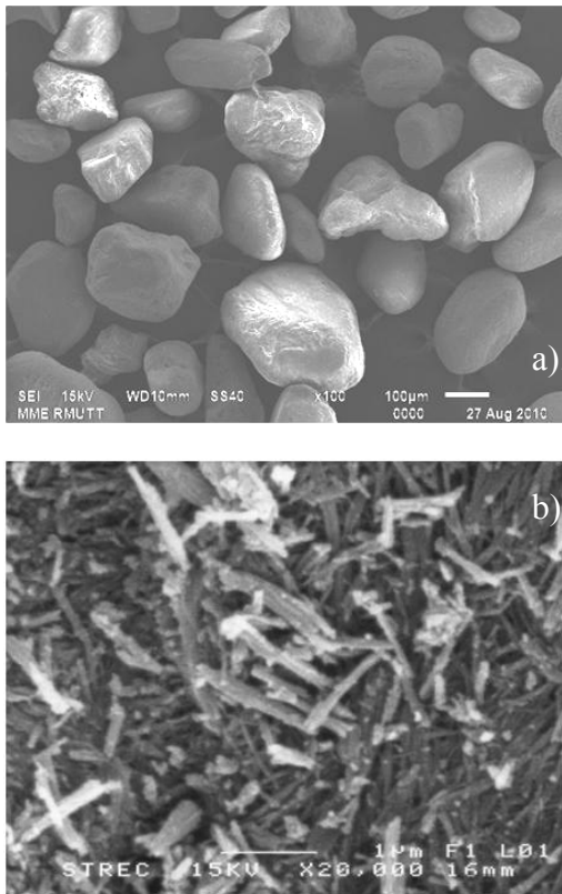
Fig. 4 SEM images of (a) Leucoxene mineral and (b) the as-synthesized sample.
